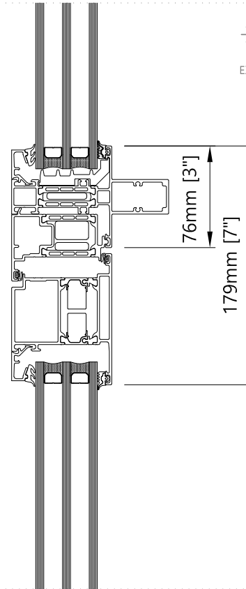
Transom - Vertical Single/Double Outswing door
