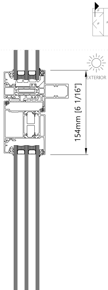
Transom - Vertical Single/Double Inswing door
