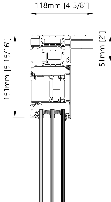
Top - Vertical Single/Double Outswing door
