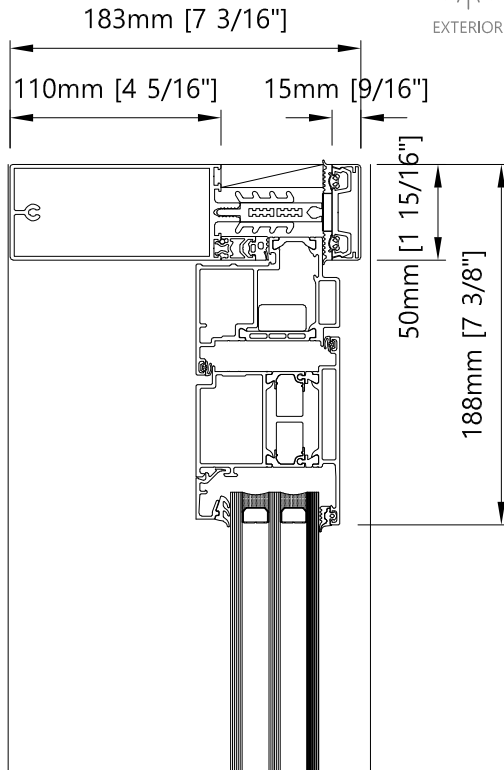
Top - Vertical Single/Double Outswing door
