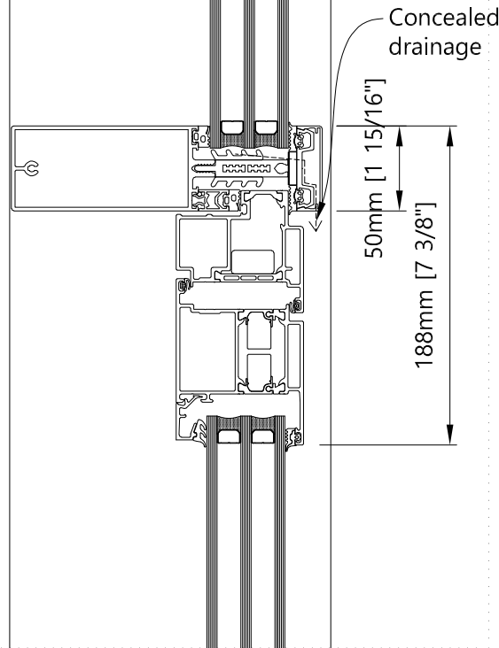
Transom - Vertical Single/Double Inswing door
