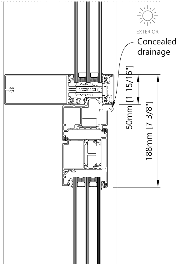
Transom - Vertical Single/Double Outswing door
