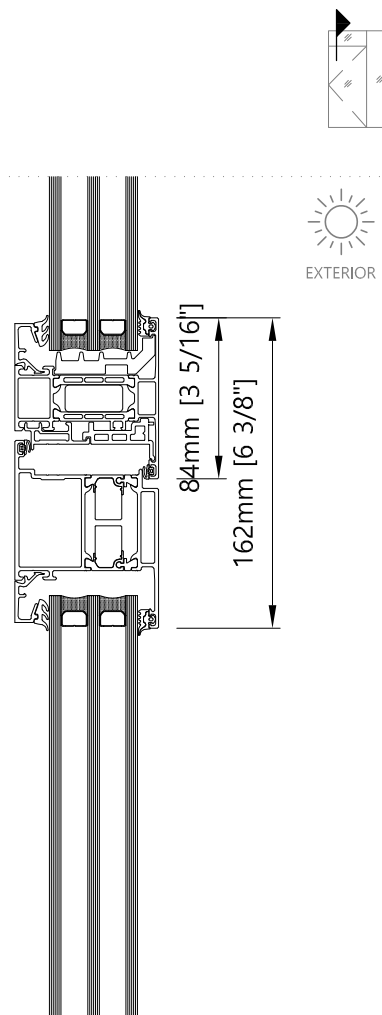
5 Transom - Vertical Single/Double Inswing door
