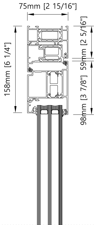
Top - Vertical Single/Double Outswing door
