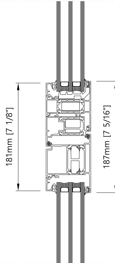
Transom - Vertical Single/Double Outswing door
