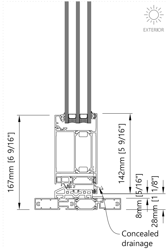
Bottom - Vertical Single/Double Outswing door
