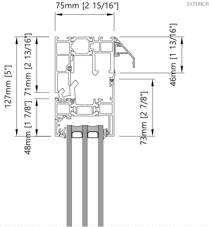
Top - Vertical Outswing bi-folding door
