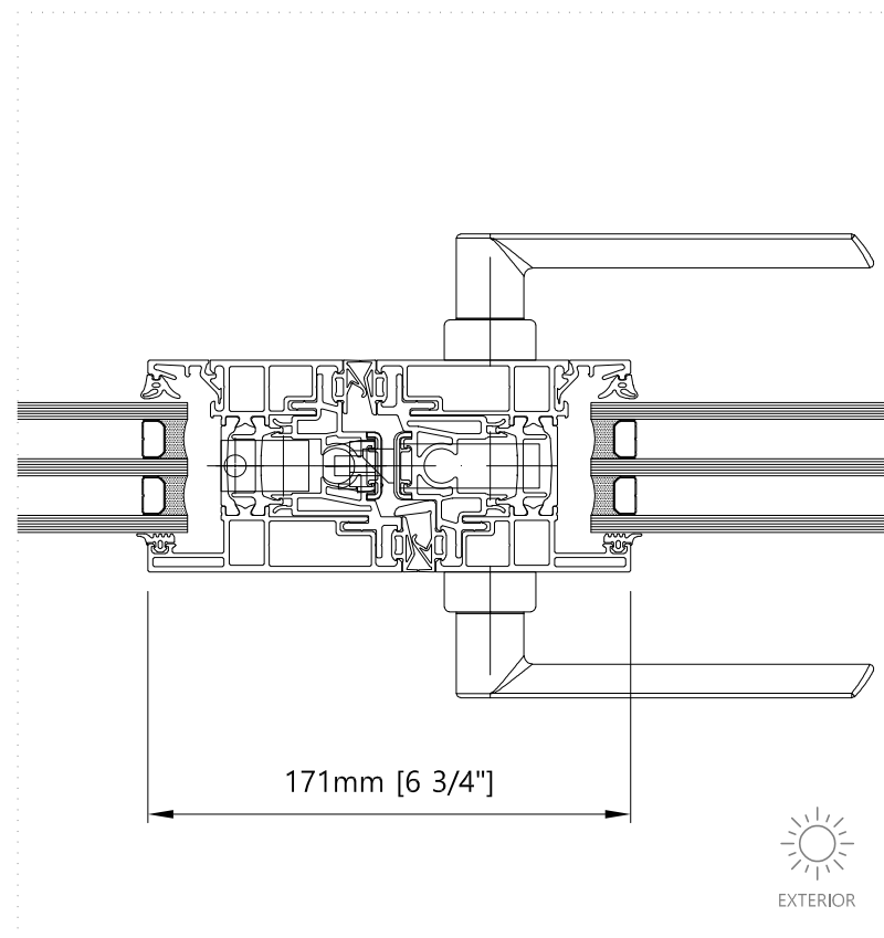
Meeting section - Horizontal Inswing bi-folding door
