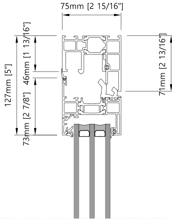
Top - Vertical Inswing bi-folding door
