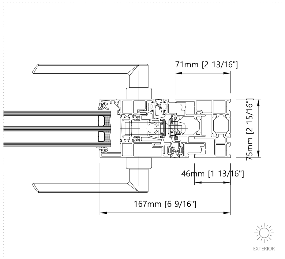
4 Jamb - Horizontal Outswing bi-folding door
