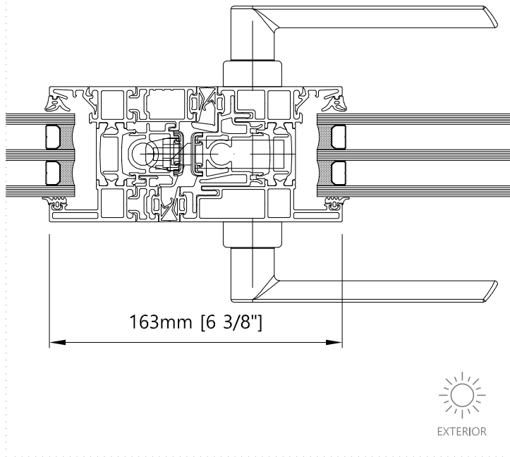
7 Meeting section - Horizontal Outswing bi-folding door
