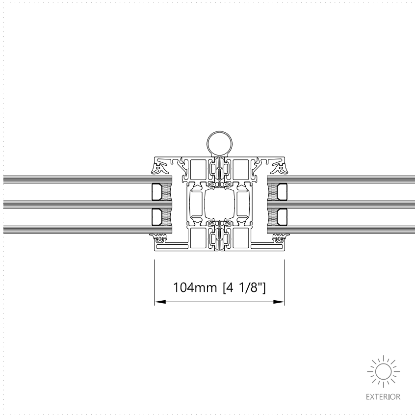
3 Meeting section - Horizontal Inswing bi-folding door
