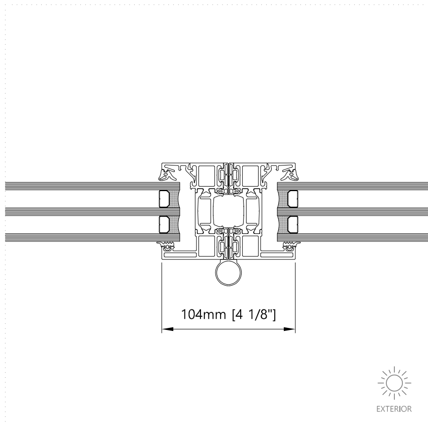
3 Meeting section - Horizontal Outswing bi-folding door
