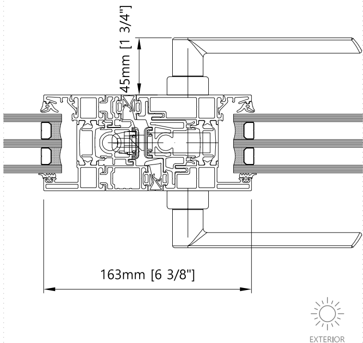
7 Meeting section - Horizontal Inswing bi-folding door
