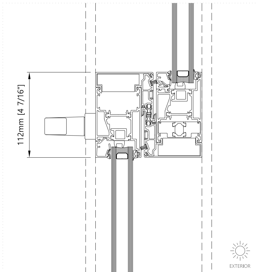
Meeting Section - Horizontal Corner Two Track L&S Door without Fly Screen
