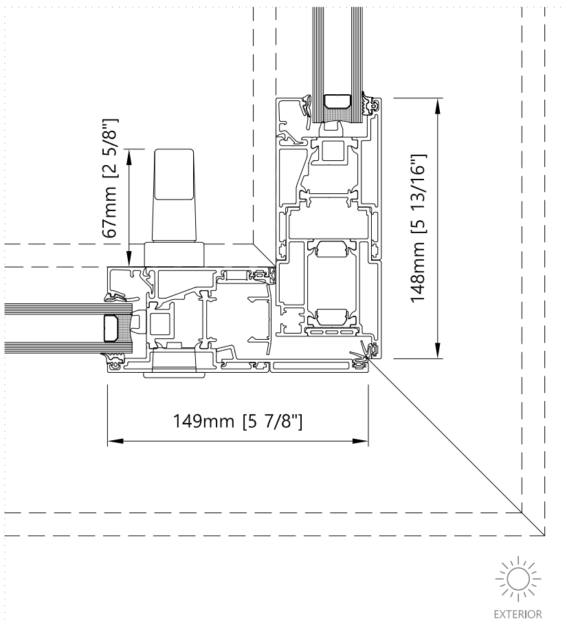
Corner Section - Horizontal Corner Two Track L&S Door without Fly Screen
