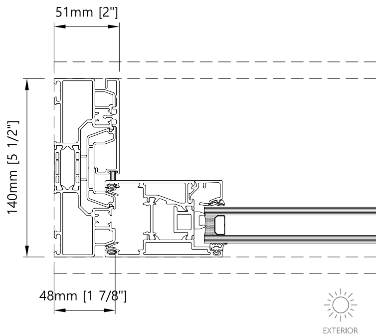
Jamb - Horizontal Corner Two Track L&S Door without Fly Screen
