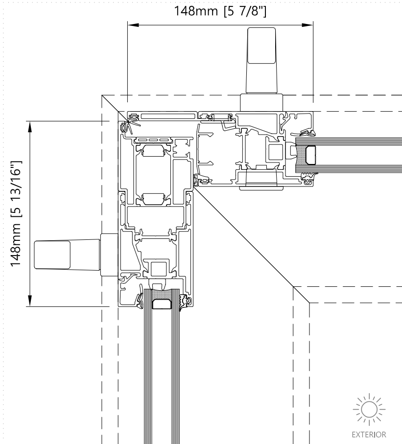
7 Corner Section - Horizontal Corner Two Track L&S Door without Fly Screen
