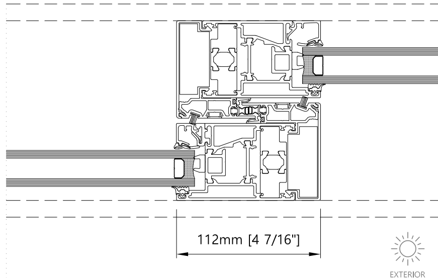
Meeting Section - Horizontal Corner Two Track L&S Door without Fly Screen
