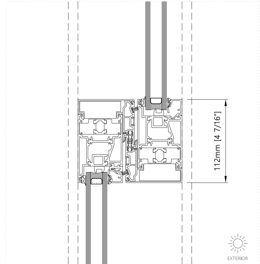
8 Meeting Section - Horizontal Corner Two Track L&S Door without Fly Screen
