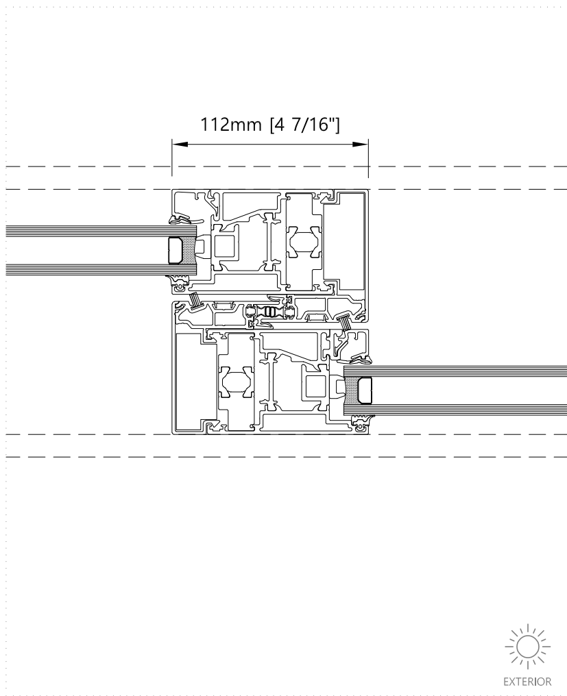
Meeting section - Horizontal Two Panel/Bi-parting L&S Door without Fly Screen
