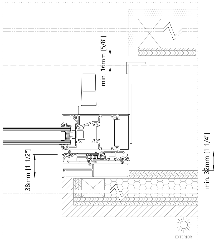
Pocket section - Horizontal Two Panel/Bi-parting L&S Door without Fly Screen
