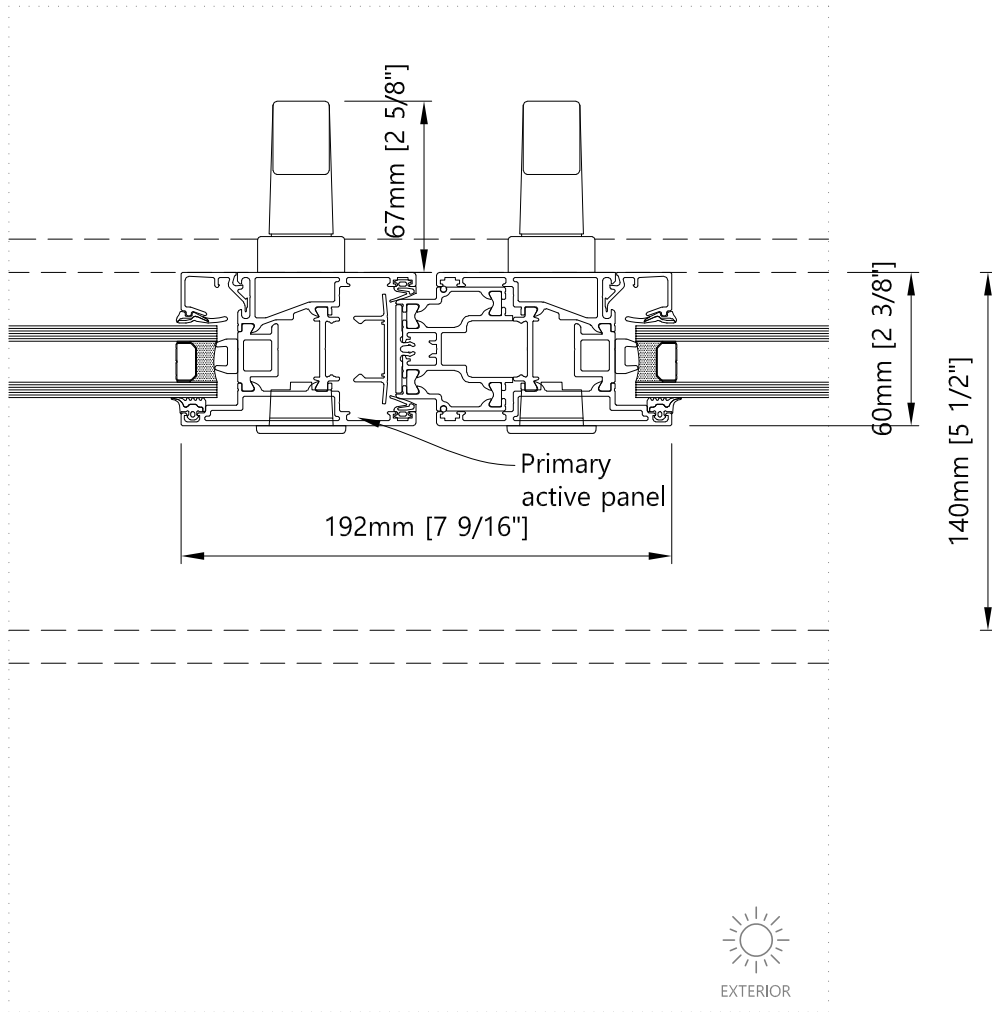
Meeting section - Horizontal Single/Two Panel Bi-parting L&S Door without Fly Screen
