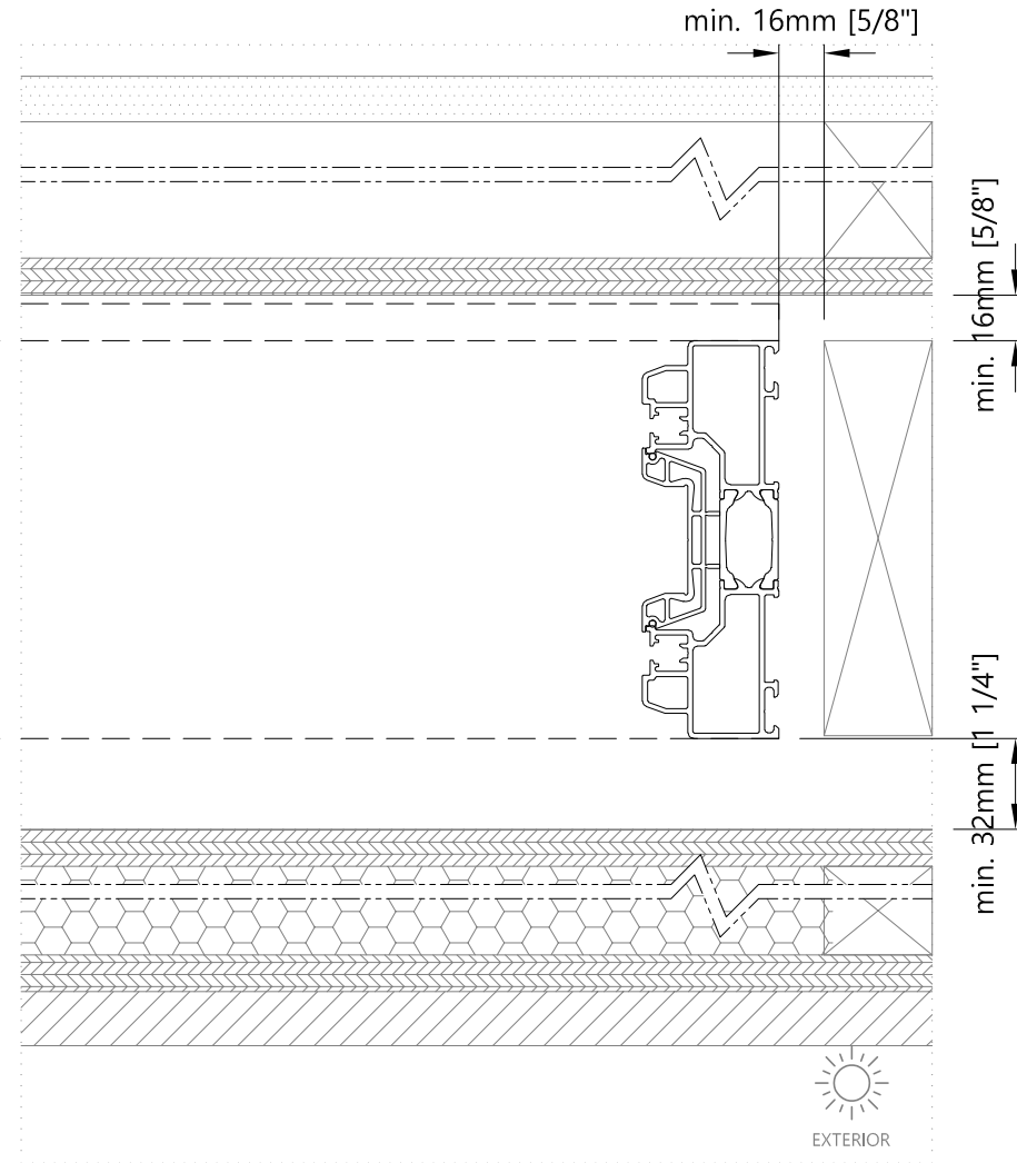
Meeting section - Horizontal Single/Two Panel Bi-parting L&S Door without Fly Screen
