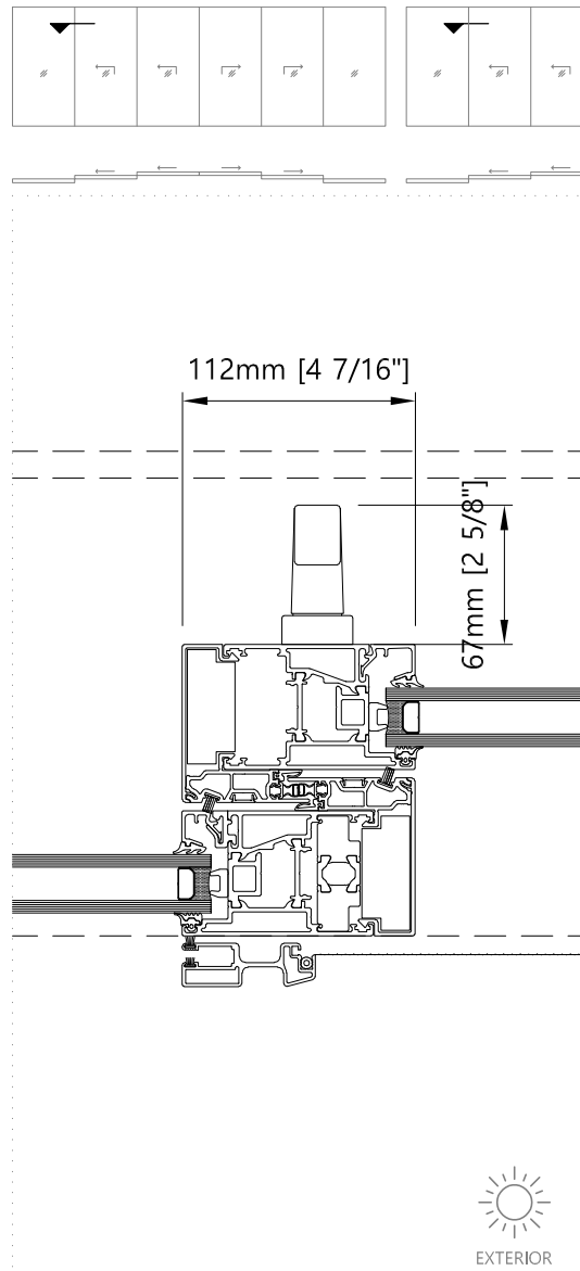
Meeting section - Horizontal Three/Six Panel L&S Door with Fly Screen
