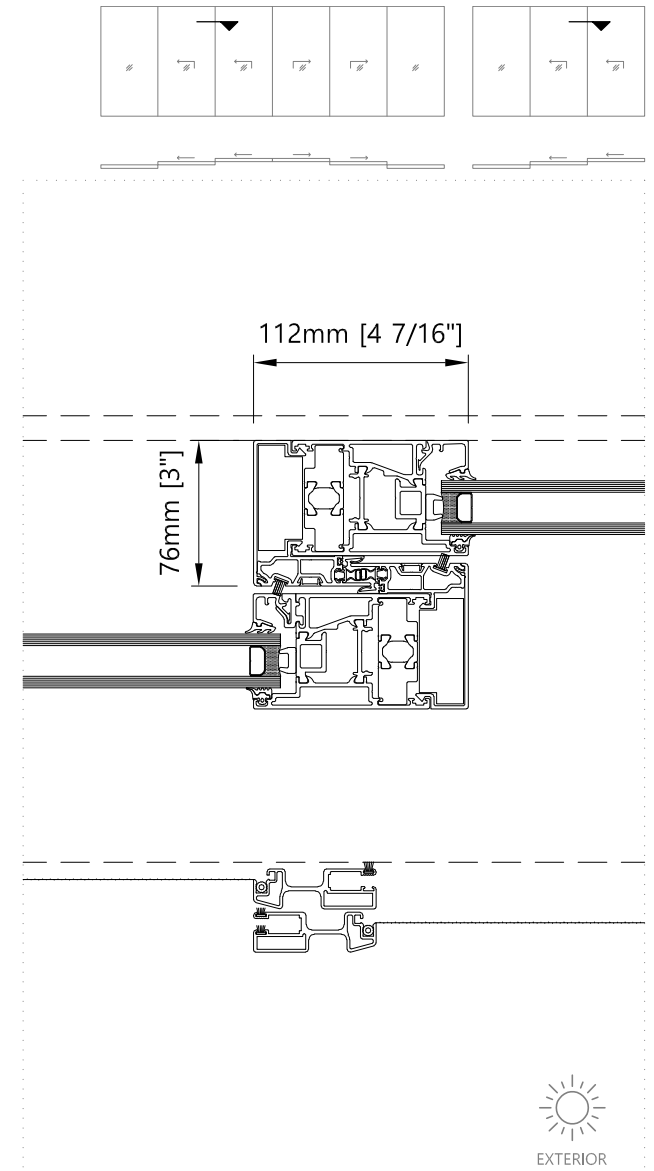
Meeting section - Horizontal Three/Six Panel L&S Door with Fly Screen
