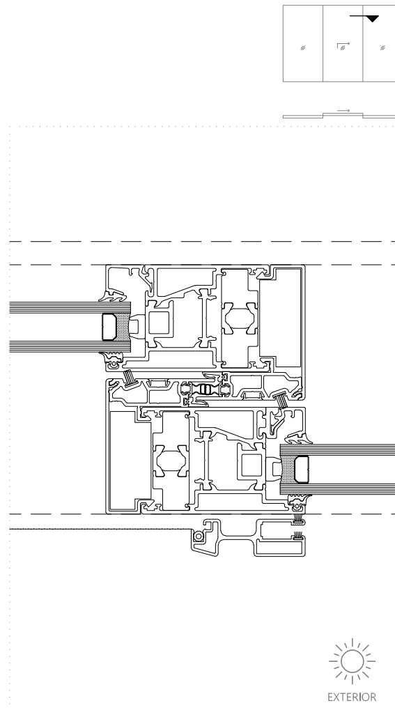
Meeting section - Horizontal Three Panel Lift & Slide Door with Fly Screen
