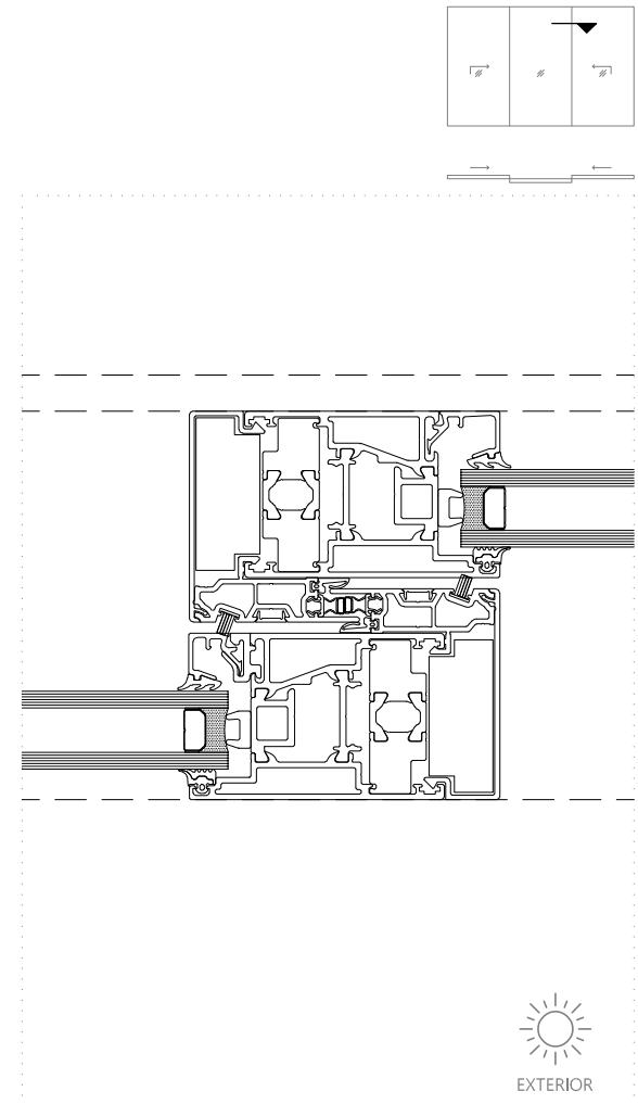
Meeting section - Horizontal Three Panel Lift & Slide Door with Fly Screen
