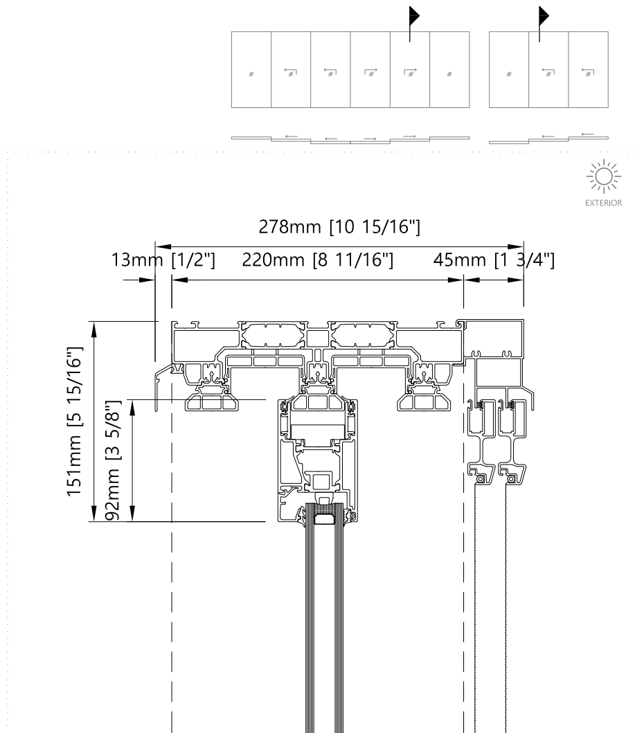
Top - Vertical Three/Six Panel Lift & Slide Door with Fly Screen
