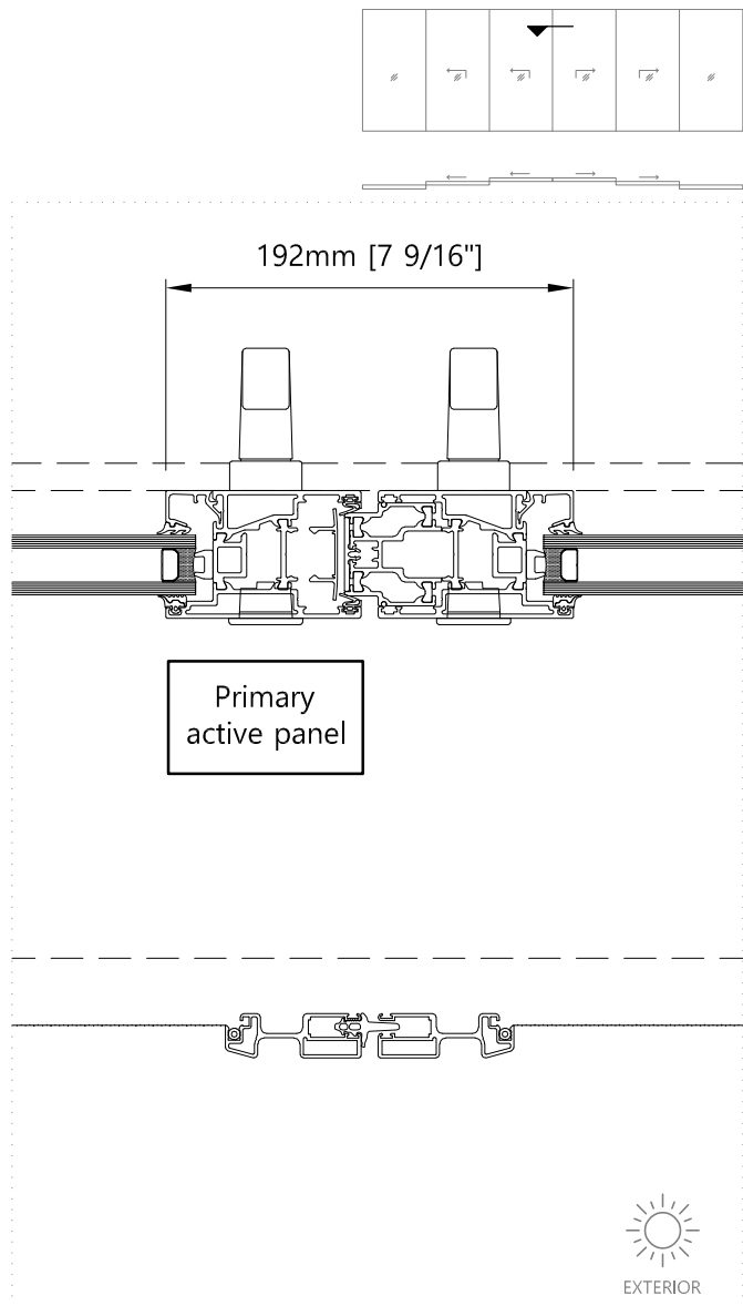
Meeting section - Horizontal Six Panel Bi-parting L&S Door with Fly Screen
