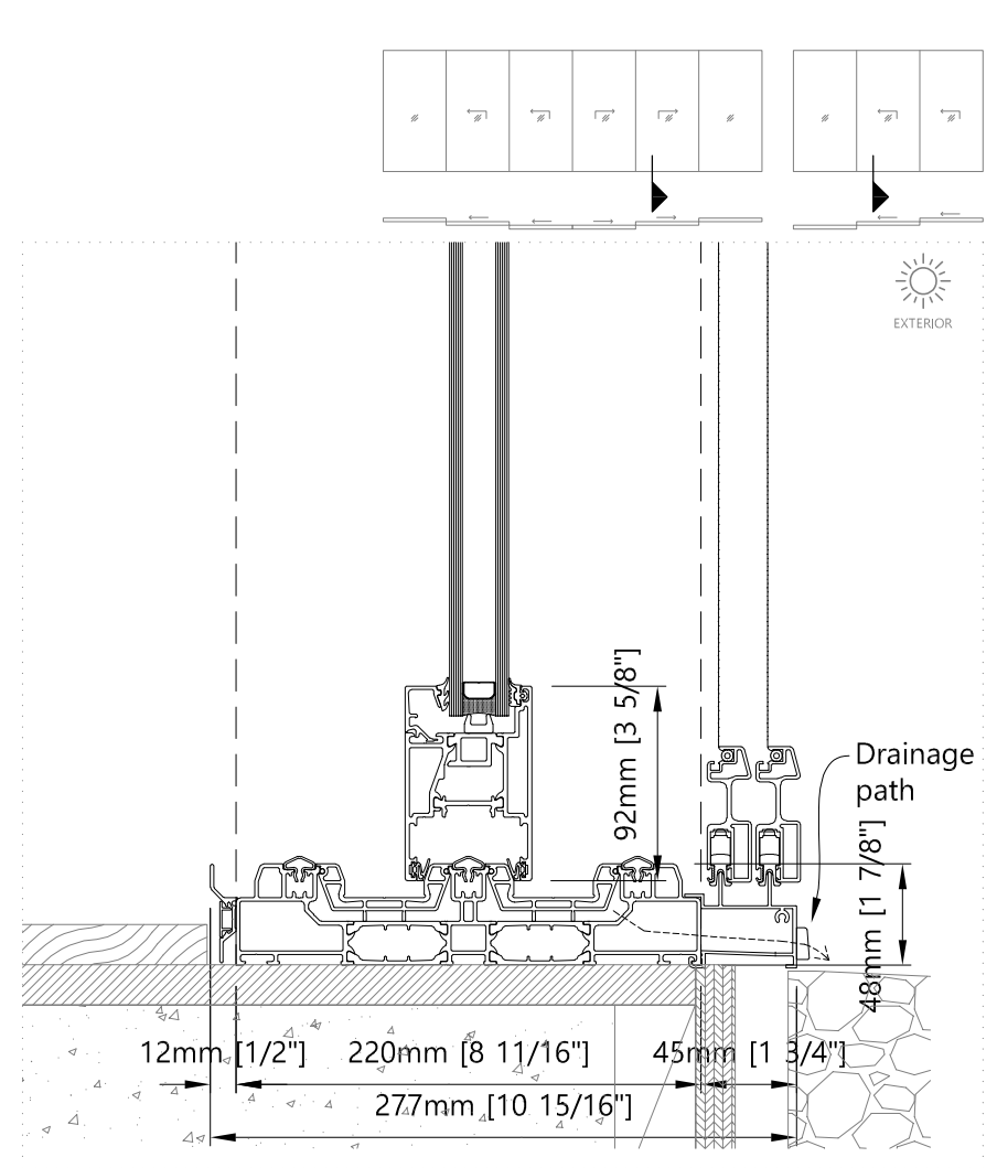
Bottom - Vertical Three/Six Panel Lift & Slide Door with Fly Screen
