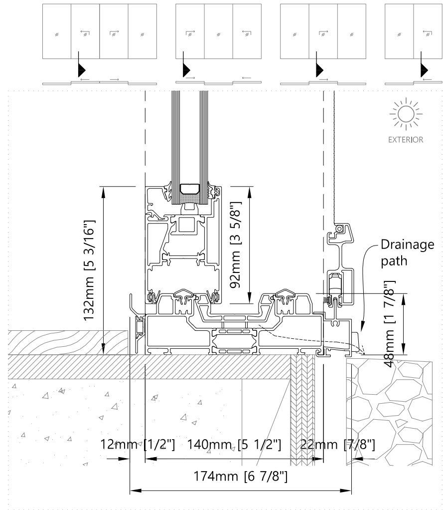
11 Bottom - Vertical Two/Three/Four Panel Lift & Slide Door with Fly Screen
