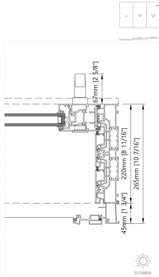
Jamb - Horizontal Three Panel L&S Door with Fly Screen
