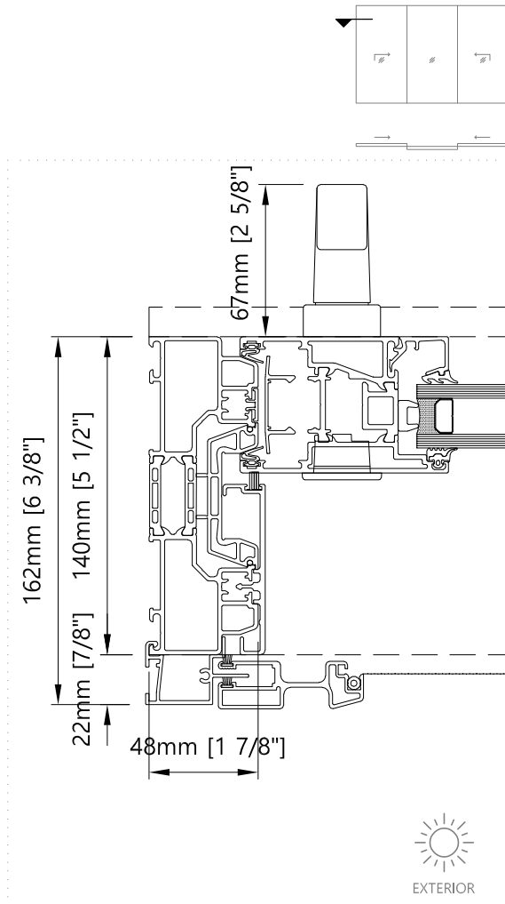
Jamb - Horizontal Three Panel Lift & Slide Door with Fly Screen
