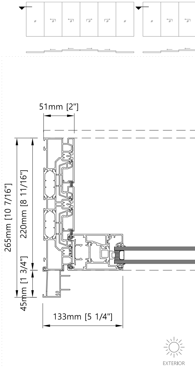
Jamb - Horizontal Three/Six Panel L&S Door with Fly Screen
