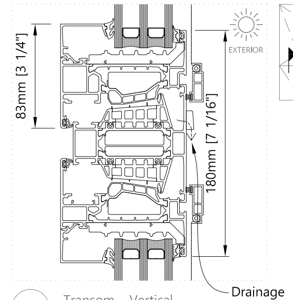
17 Transom - Vertical Motorized hopper window
