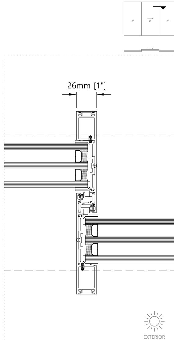
9 Meeting section - Horizontal Sliding Door without Fly Screen
