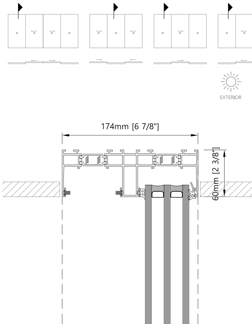
Top - Vertical Sliding Door without Fly Screen
