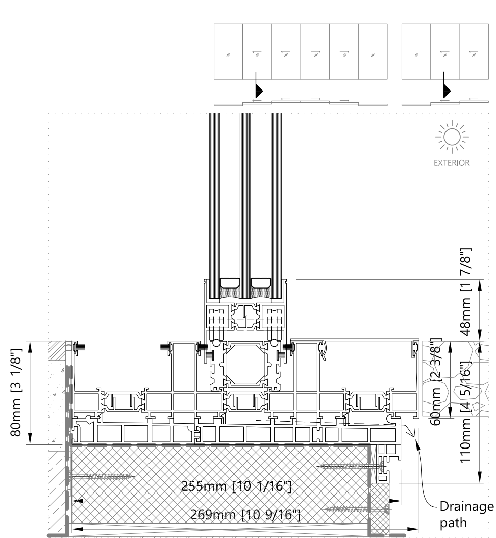
Bottom - Vertical Sliding Door without Fly Screen
