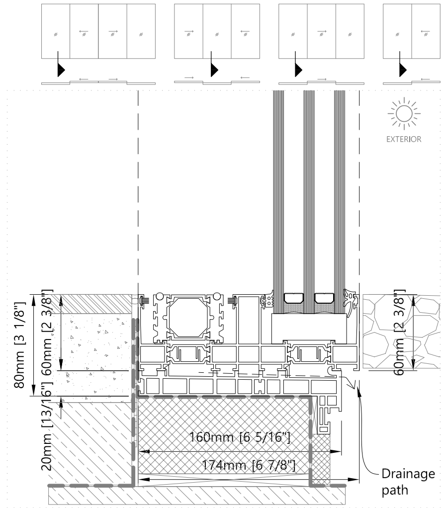
Bottom - Vertical Sliding Door without Fly Screen
