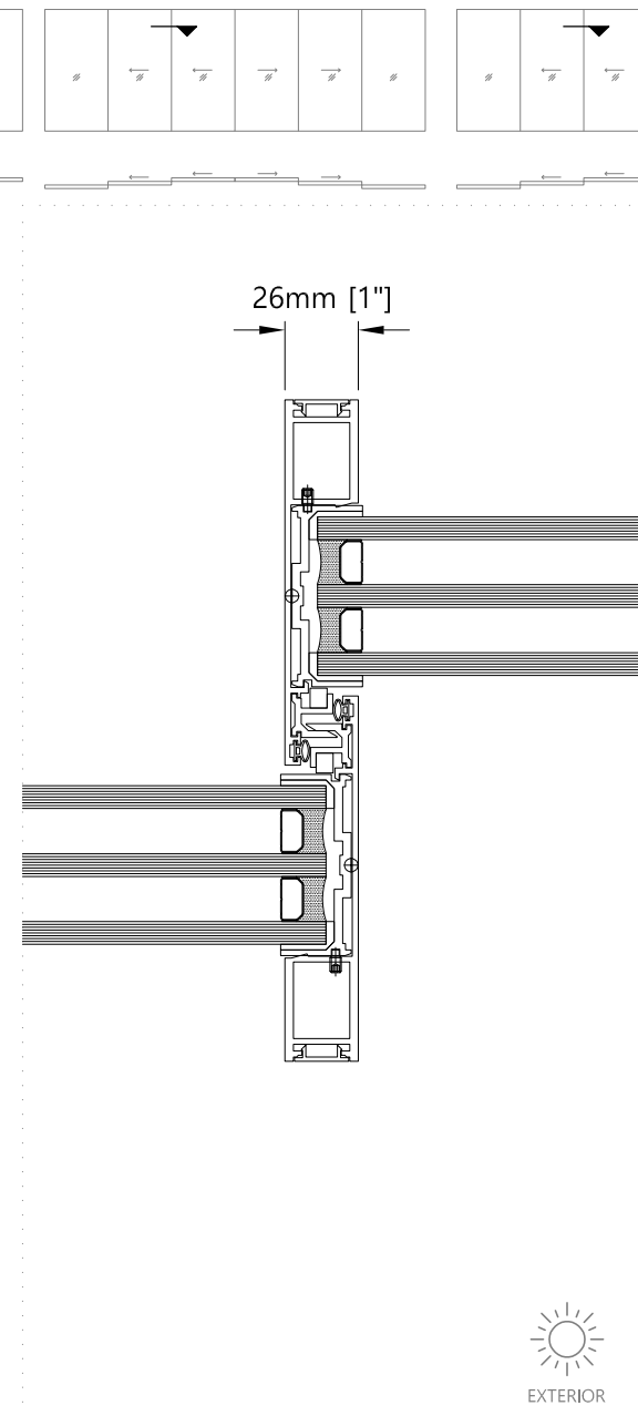
Meeting section - Horizontal Sliding Door without Fly Screen
