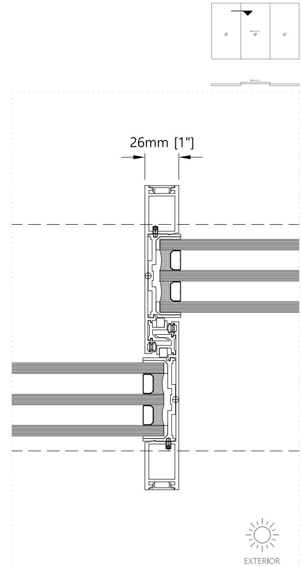
10 Meeting section - Horizontal Sliding Door without Fly Screen
