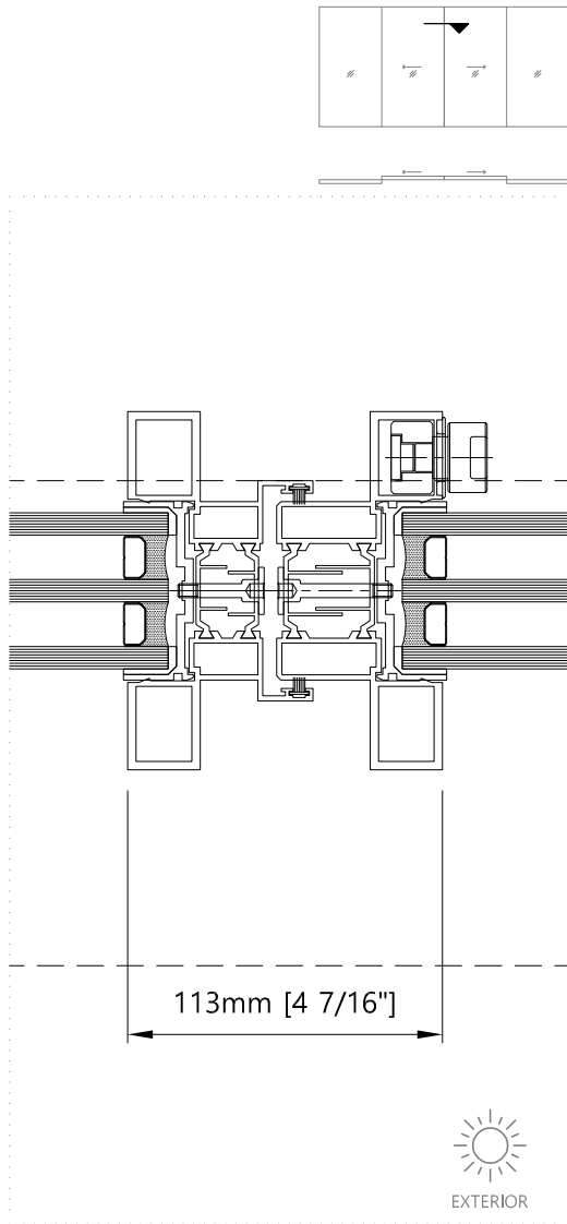
4 Meeting section - Horizontal Sliding Bi-Parting Door without Fly Screen
