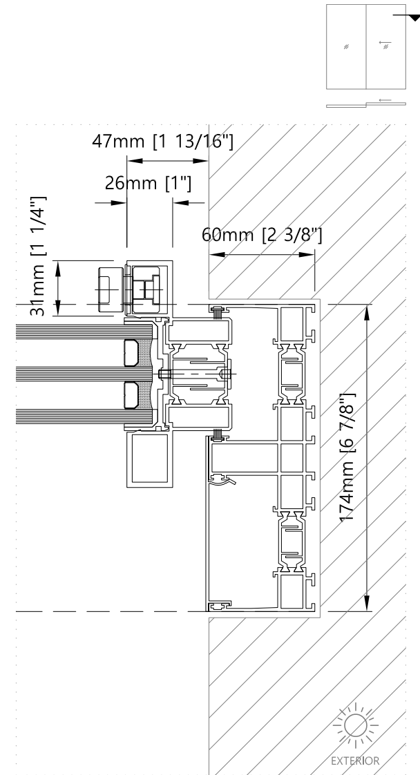
3 Jamb - Horizontal Sliding Door without Fly Screen
