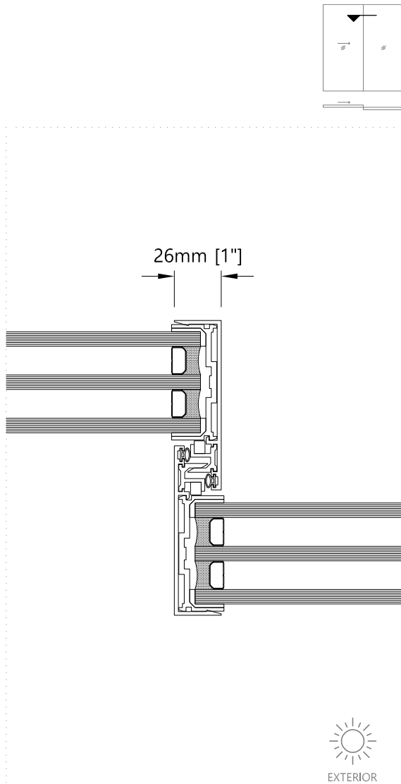
X Interlock option 1 Sliding Door without Fly Screen
