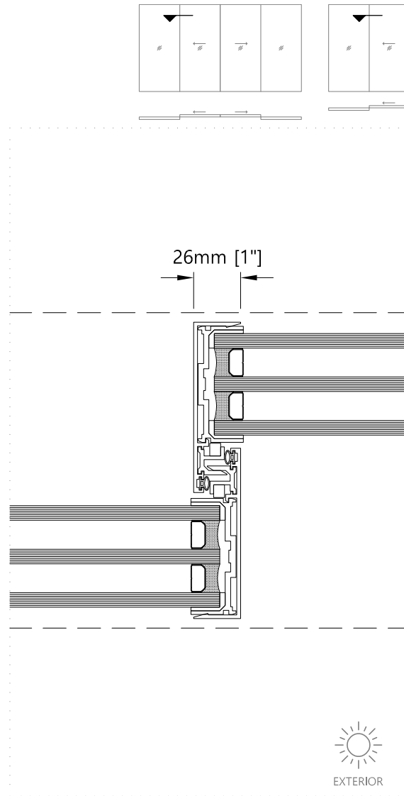
2 Meeting section - Horizontal Sliding Door without Fly Screen
