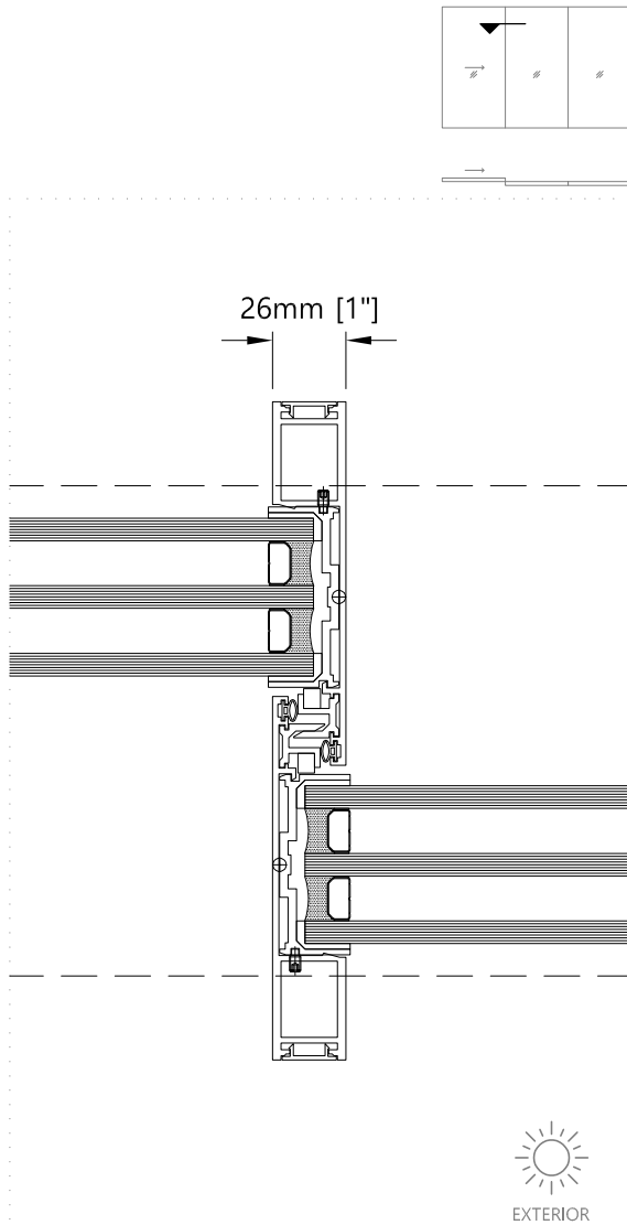
Meeting section - Horizontal Sliding Door without Fly Screen
