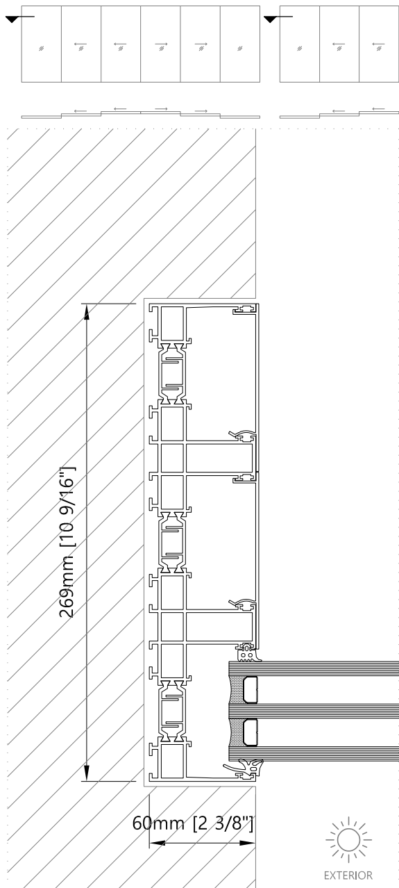
Jamb - Horizontal Sliding Door without Fly Screen
