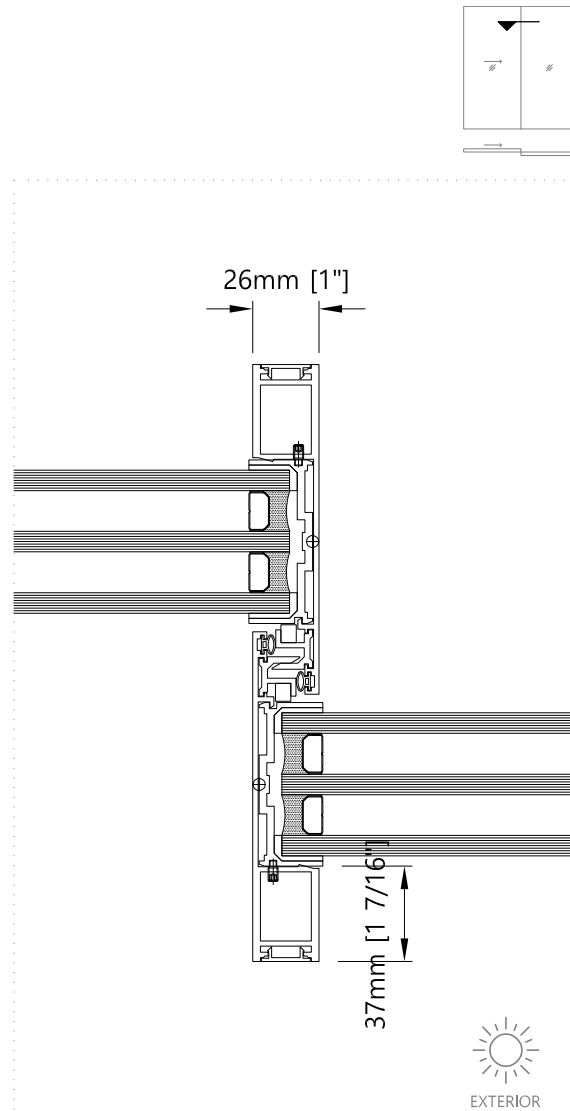
X Interlock option 2 Sliding Door without Fly Screen
