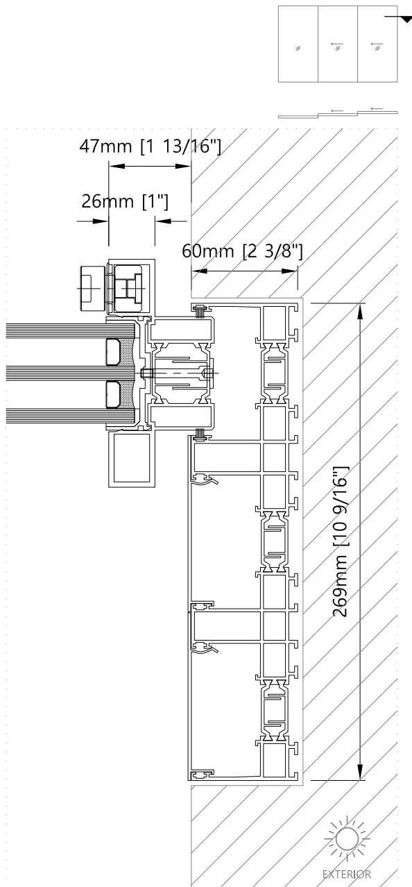
18 Jamb - Horizontal Sliding Door without Fly Screen
