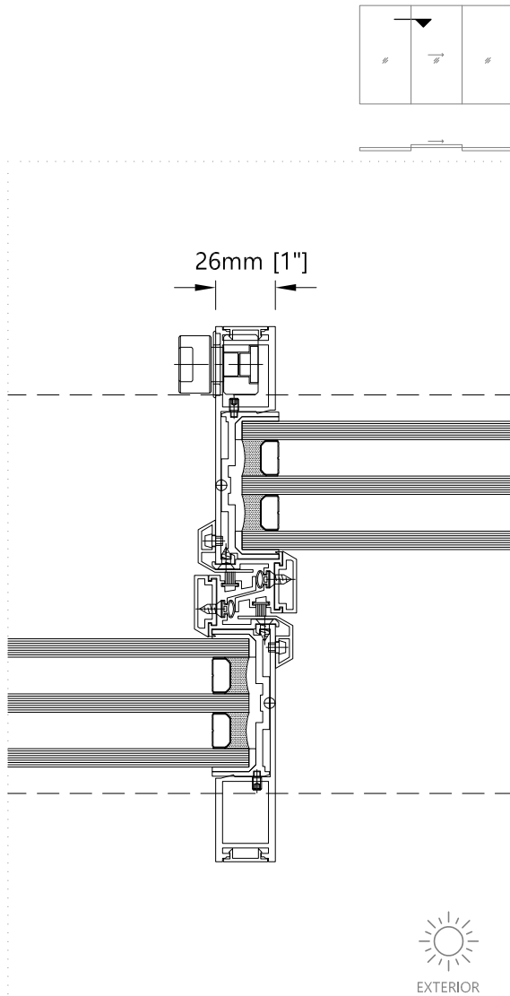
8 Meeting section - Horizontal Sliding Door without Fly Screen
