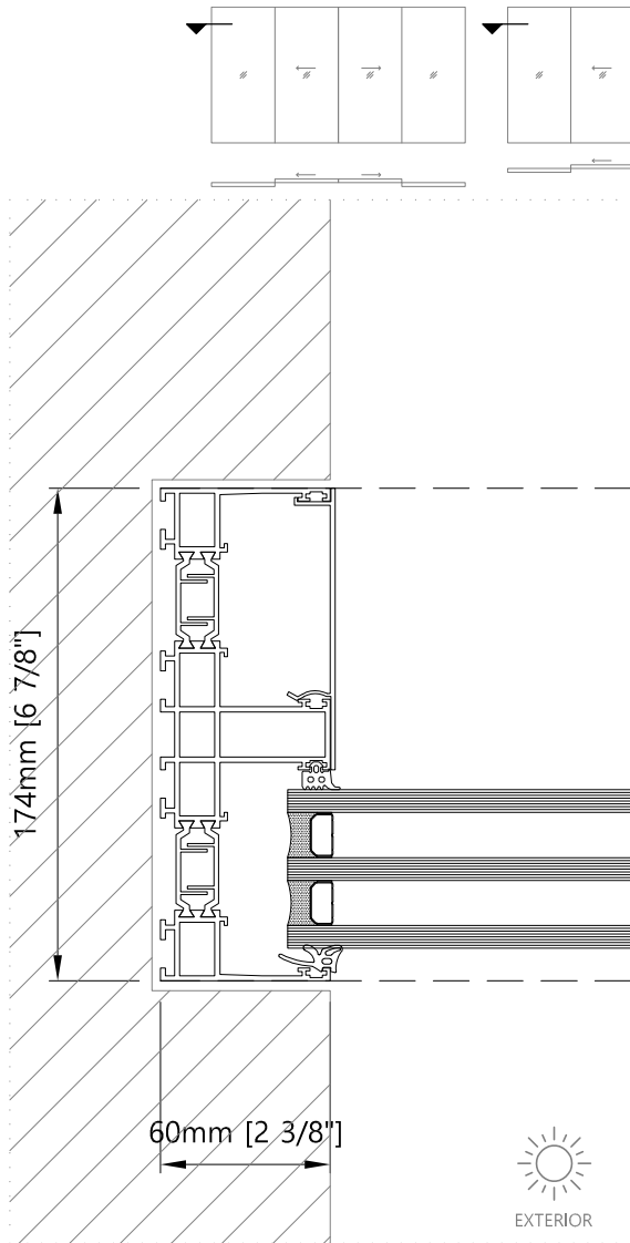
1 Jamb - Horizontal Sliding Door without Fly Screen
