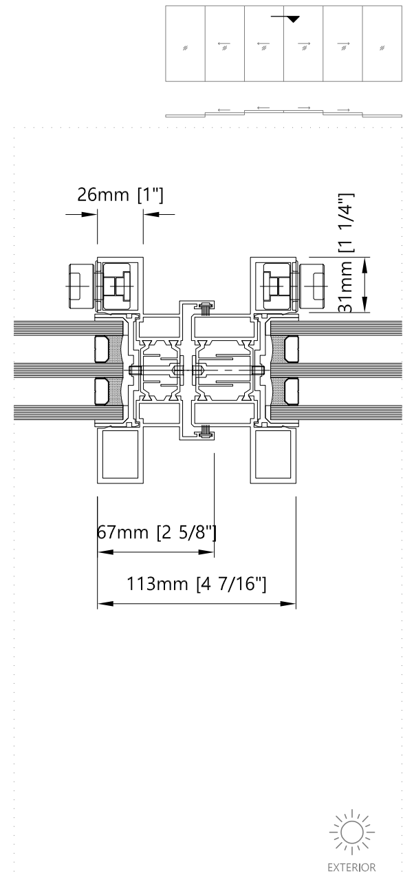
19 Meeting section - Horizontal Sliding Door without Fly Screen
