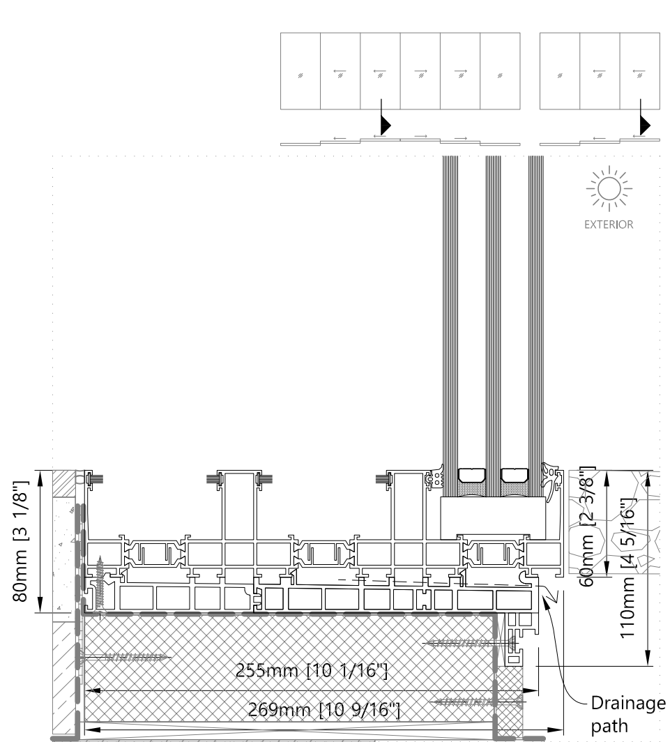
Bottom - Vertical Sliding Door without Fly Screen
