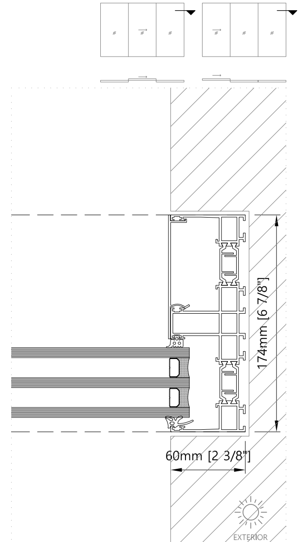
Jumb - Horizontal Sliding Door without Fly Screen
