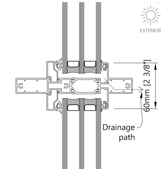
3 Transom - Vertical Fixed Window
