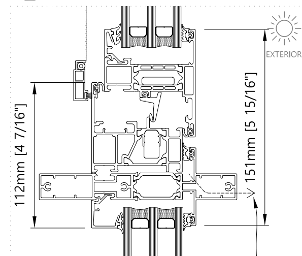
Transom - Vertical Motorized awning
