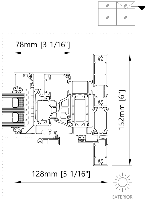
11 Jamb - Horizontal Motorized hopper
