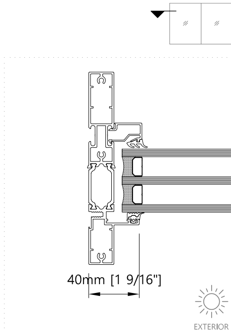
1 Jamb - Horizontal Fixed Window
