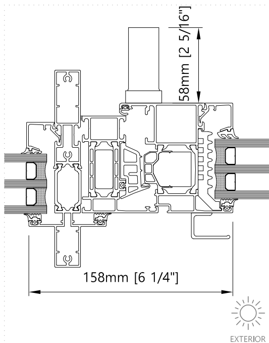
Mullion - Horizontal Single terrace door
