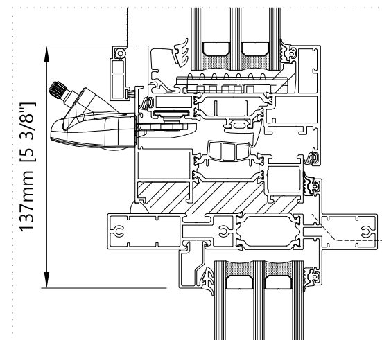
Transom - Vertical Fixed Window
