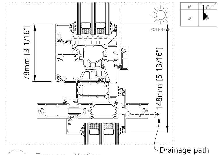
13 Transom - Vertical Motorized hopper
