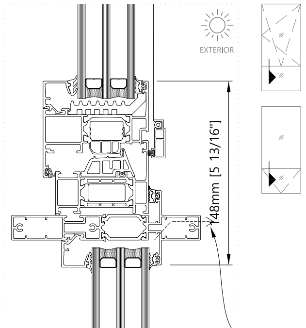
Transom - Vertical T&T Window / Double T&T
