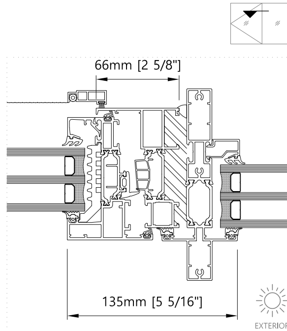
Mullion - Horizontal Fixed Window
