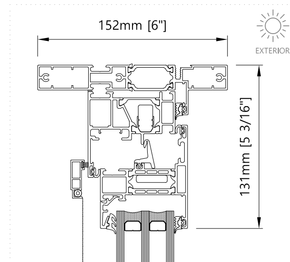
Top - Vertical Motorized awning
