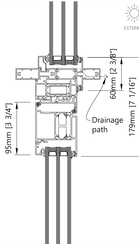
Transom - Vertical Single/Double Inswing door
