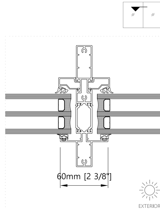
2 Mullion - Horizontal Fixed Window
