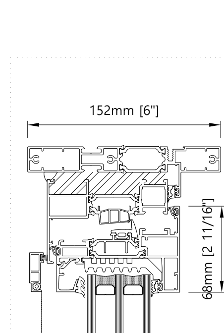
Top - Vertical Fixed Window
