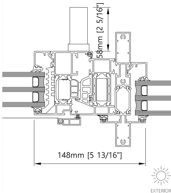
Mullion - Horizontal T&T Window / Double T&T
