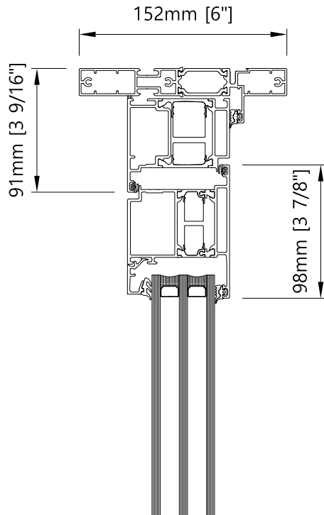
Top - Vertical Single/Double Outswing door
