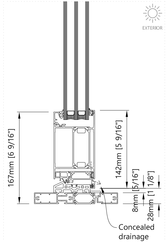
Bottom - Vertical Single/Double Outswing door
