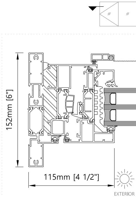
Jamb - Horizontal Fixed Window
