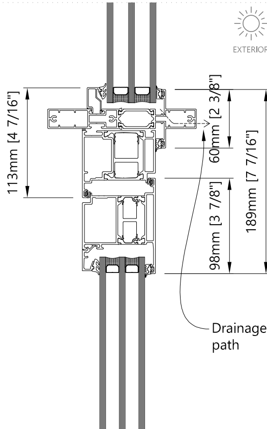
Transom - Vertical Single/Double Outswing door
