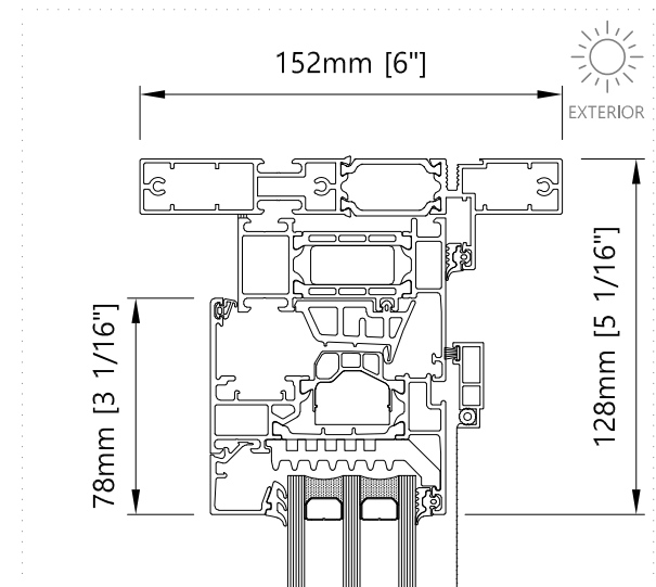
12 Top - Vertical Motorized hopper
