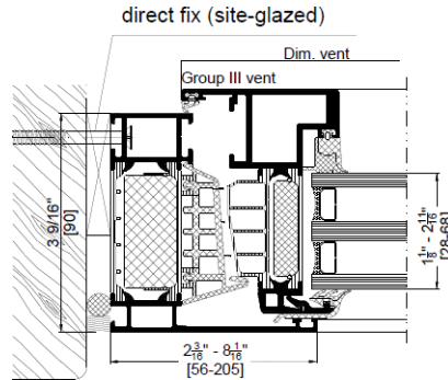
AWS 90 BS.SI+ medium vent
