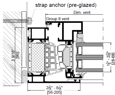
AWS 90 BS.SI+ small vent
