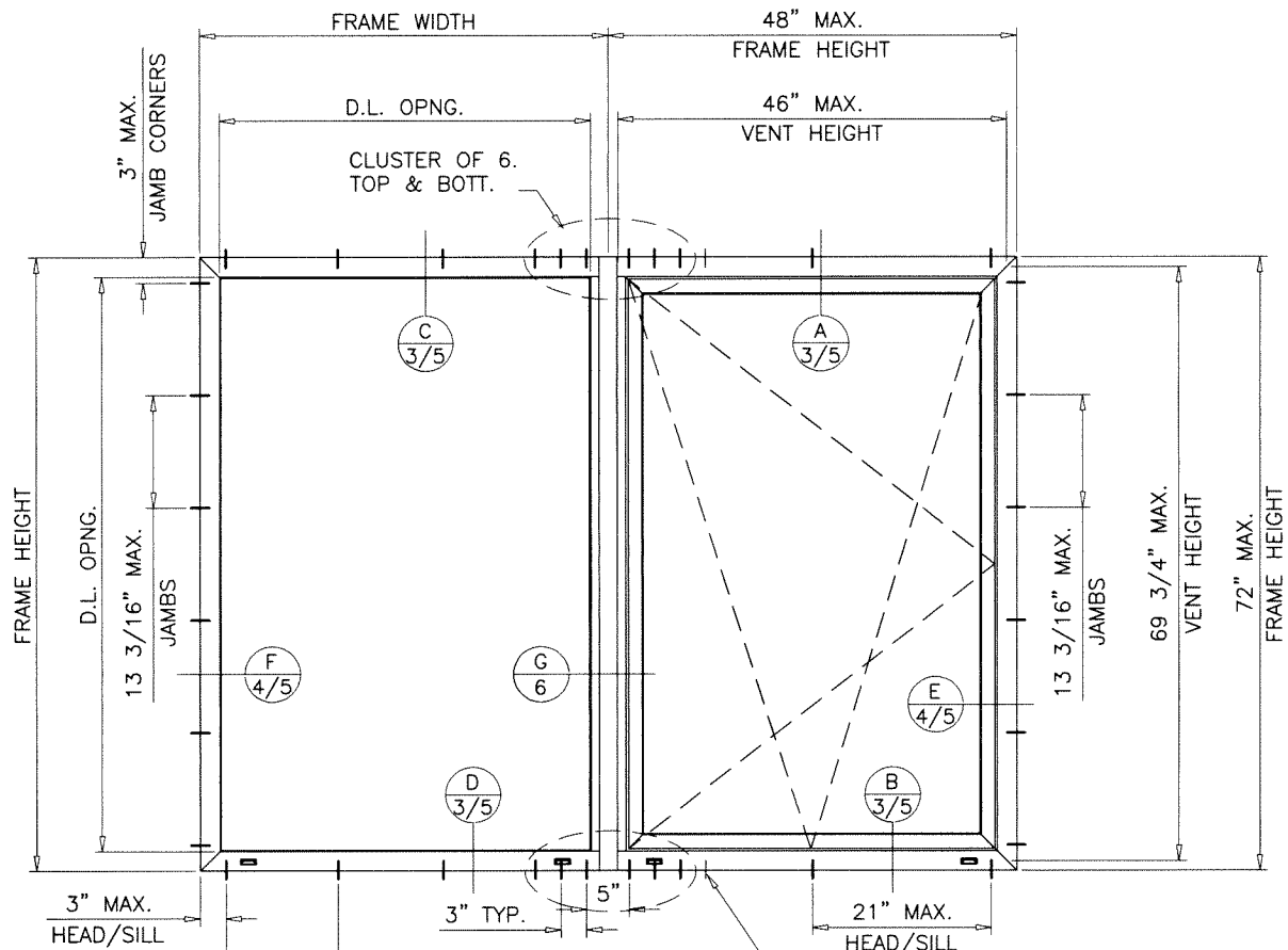
( OX ) TYPICAL ELEVATION TESTED UNIT
