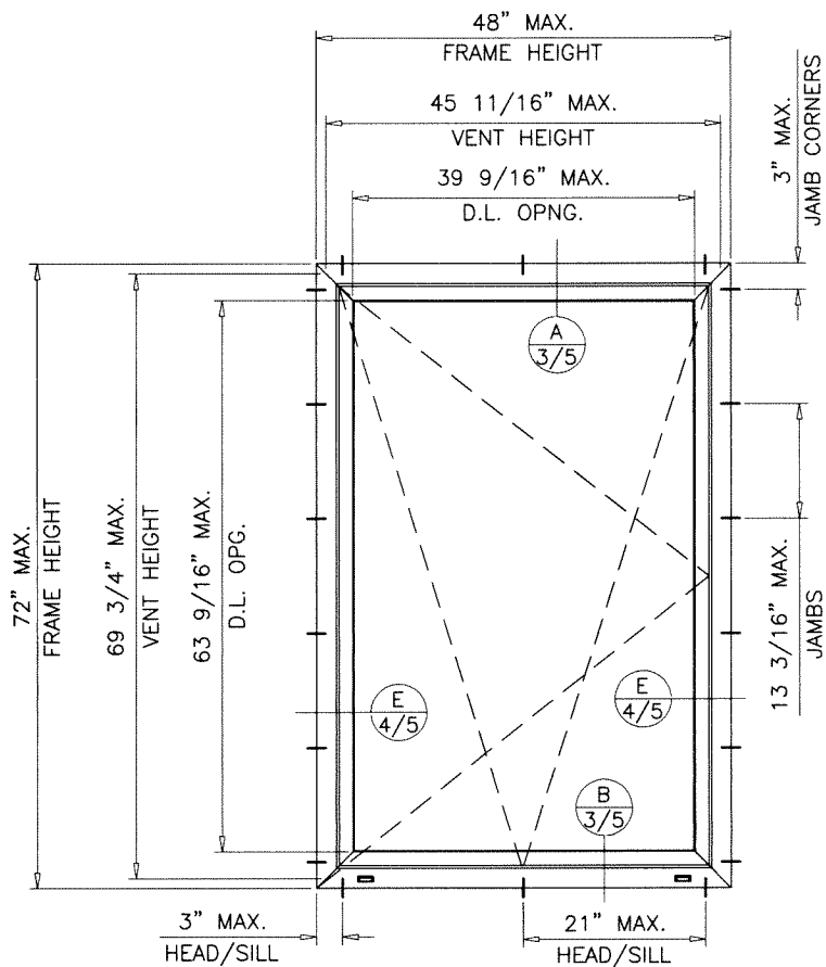
( X ) TYPICAL ELEVATION TESTED UNIT
