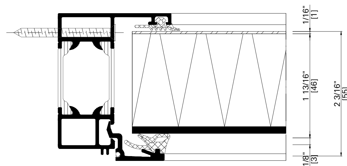
Flush Metal Spandrel Panel. 1 \frac{13}{16} " Option
