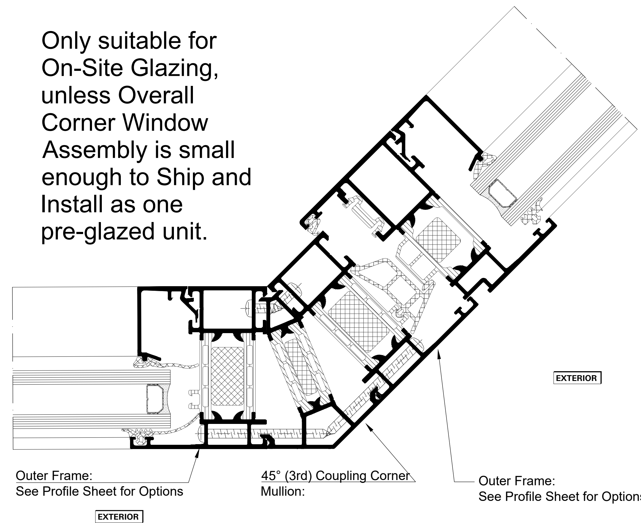
Detail 29 45° External (3rd) Coupling Corner Mullion
