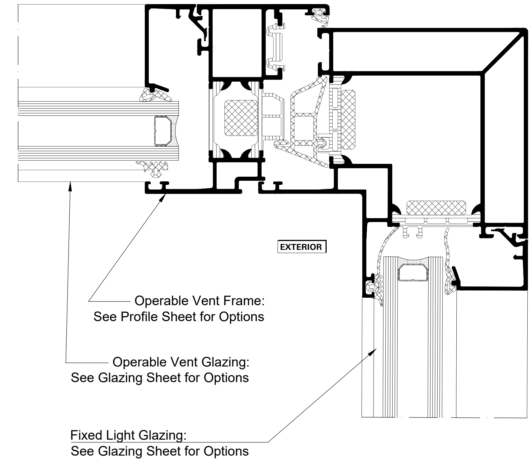
Detail 27 90° Intermediate Internal Corner Mullion
