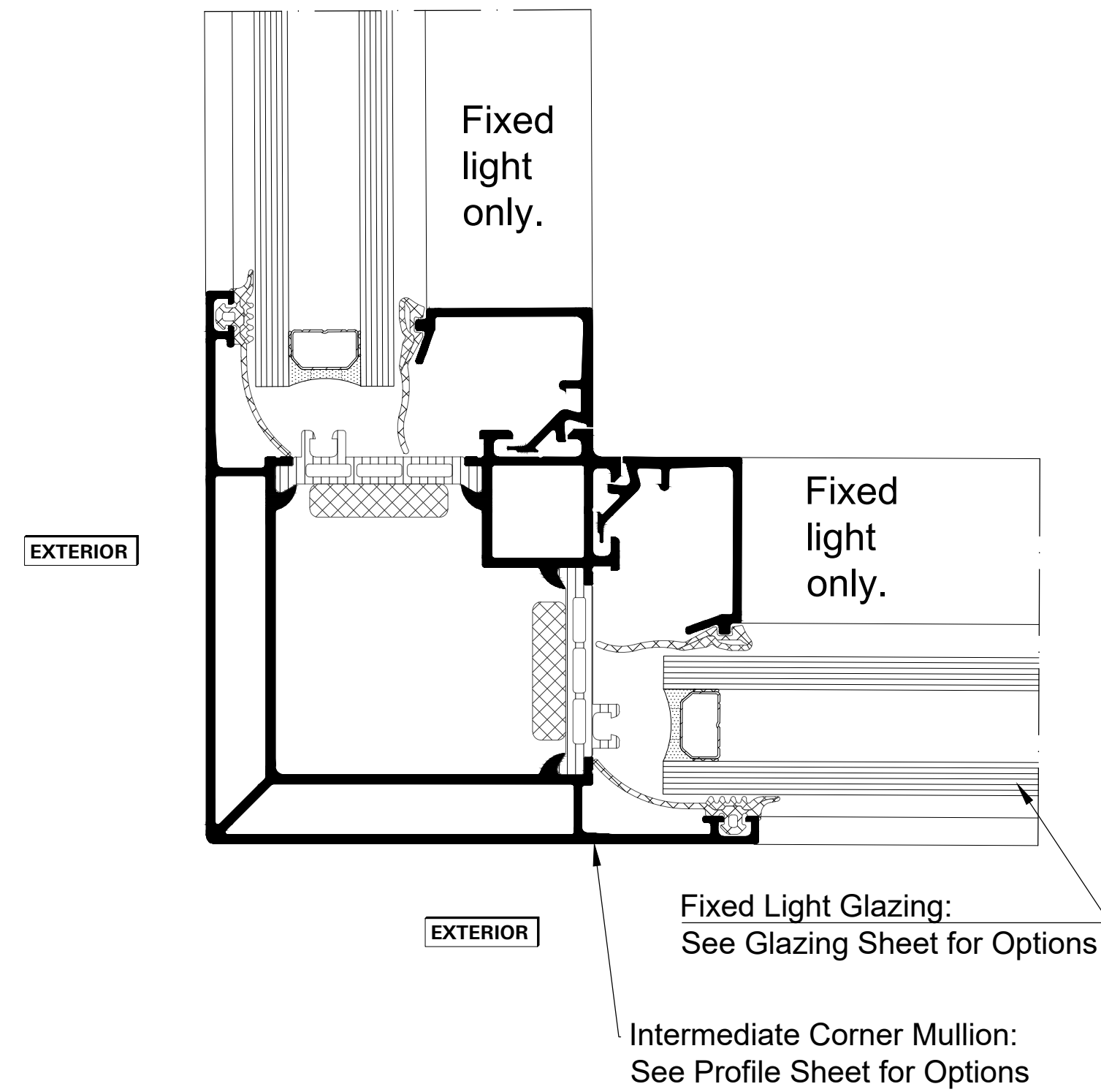
Detail 25 90° Intermediate External Corner Mullion
