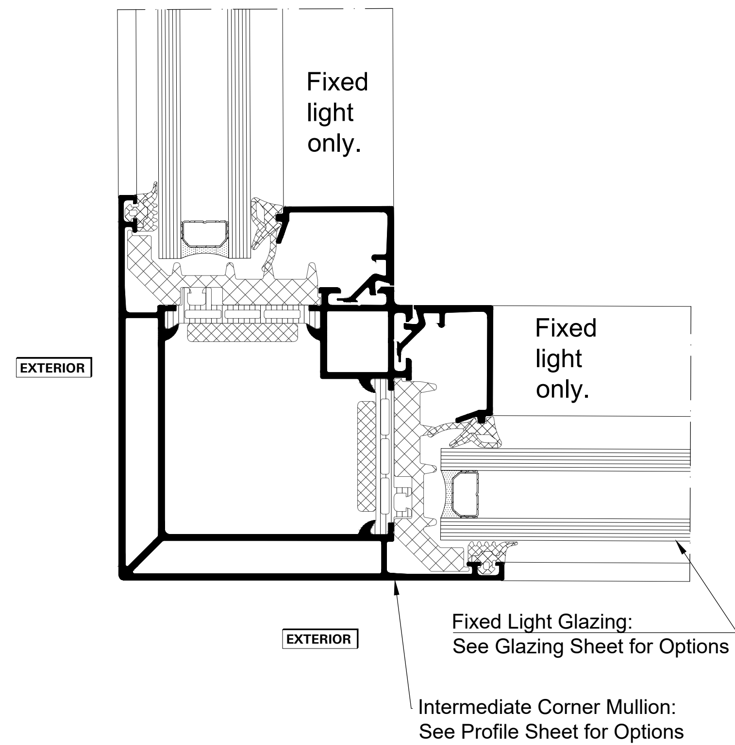
Detail 25 90° Intermediate External Corner Mullion
