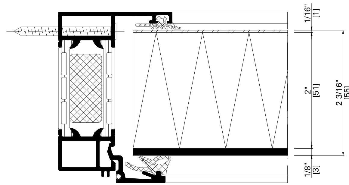
Flush Metal Spandrel Panel. 2 \frac{3}{16} " Option
