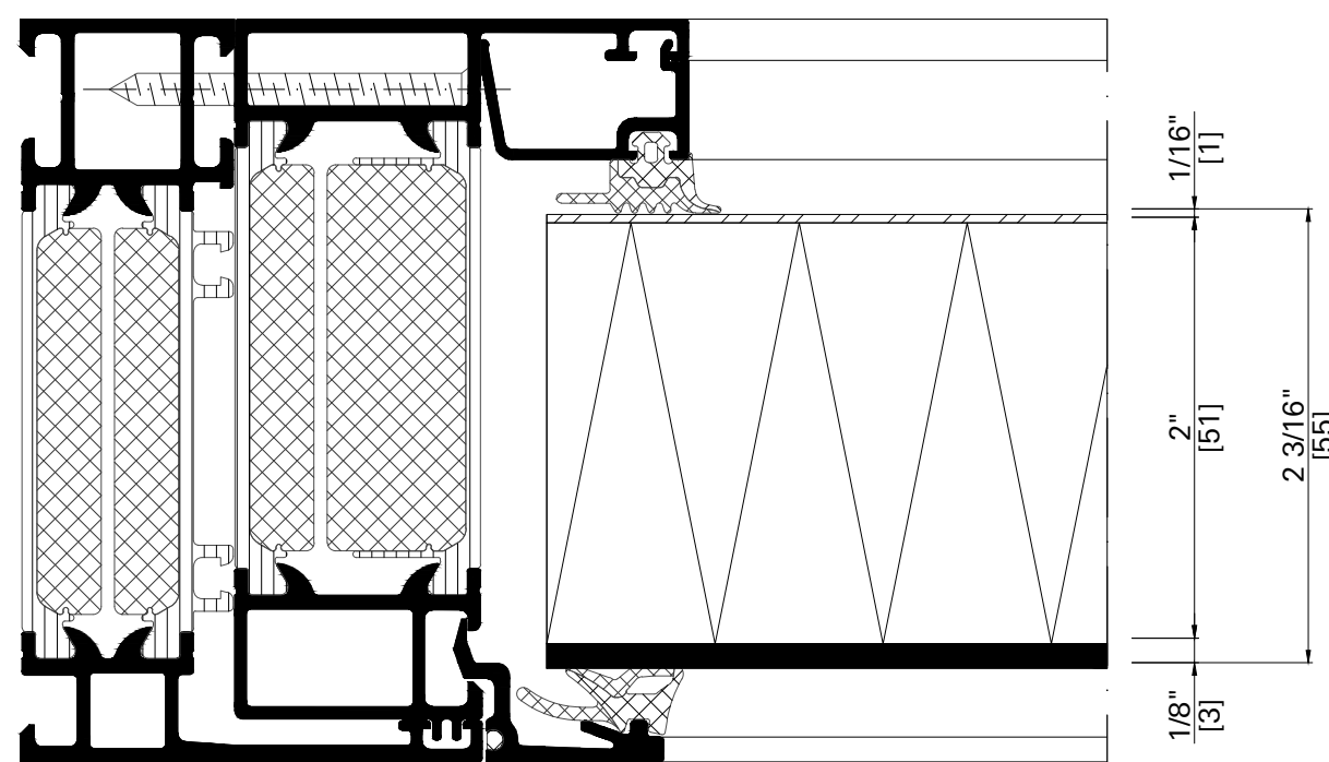
Flush Metal Spandrel Panel. 2 \frac{3}{16} " Option
