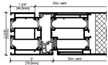
AD UP 75 Panel Door
