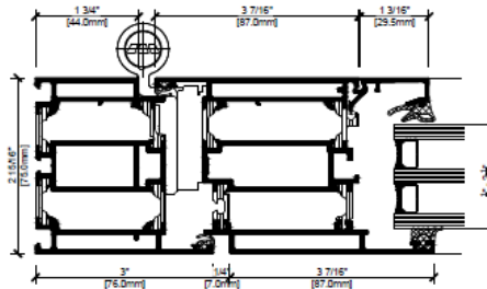
AD UP 75 BL (Basic Line) Jamb
