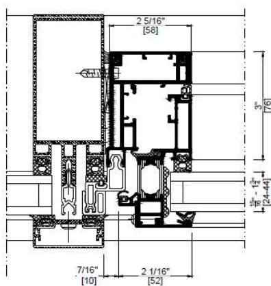
AWS 114 TipTronic
