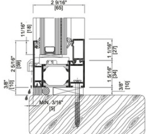
AWS 65 Sill Details
