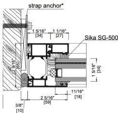
AWS 65 - Structural Mullion
