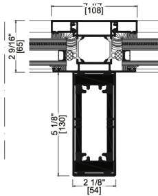
AWS 65 - Structural Mullion
