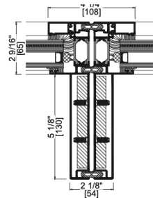
AWS 65 Couplin Mullion
