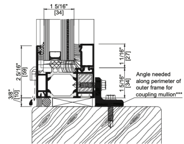
AWS 65 Coupling Mullion Sill
