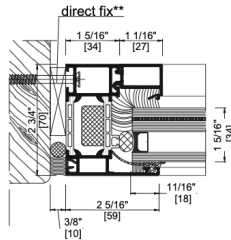
AWS 65 Couplin Mullion
