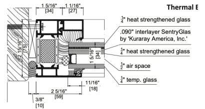
AWS 65 Coupling Mullion Sill
