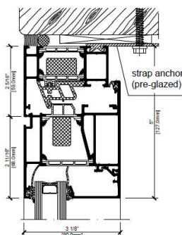
AWS 70.HI head
