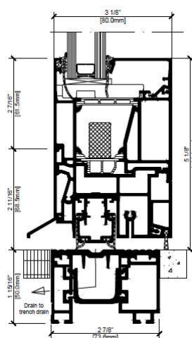
AWS 70.HI standard sill
