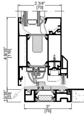
AWS 70.HI ADA threshold
