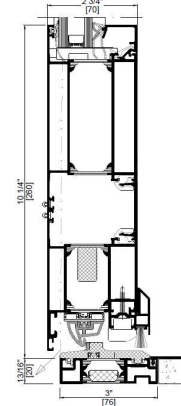
AWS 70.HI 10" Bottom Rail
