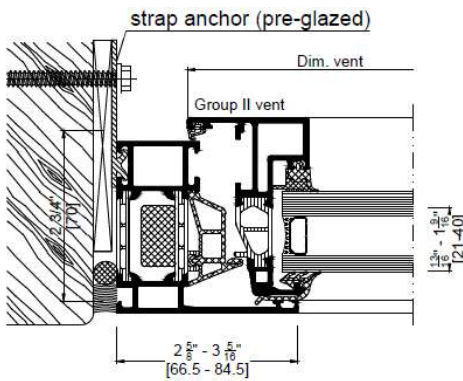
AWS 70 BS.HI small vent
