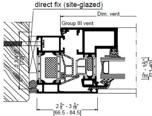
AWS 70 BS.HI small vent
