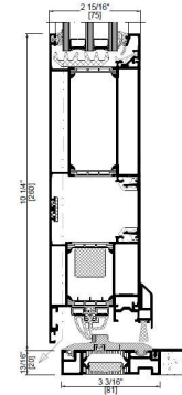
AWS 75.SI+ 10\" Bottom Rail
