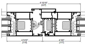
AWS 75.SI+ meeting stile
