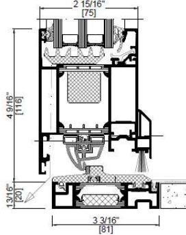
AWS 75.SI+ std ADA threshold
