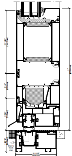
AWS 90.SI+ 10" Bottom Rail
