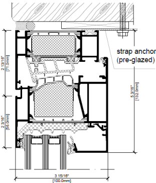
AWS 90.SI+ head
