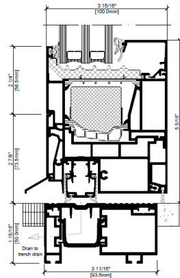
AWS 90.SI+ standard sill
