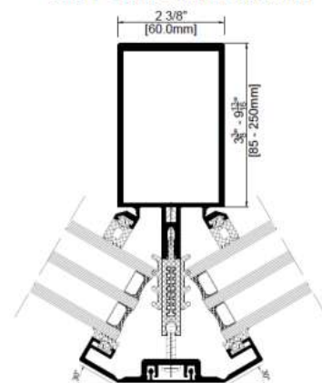
FWS 60.SI Corner Mullion
