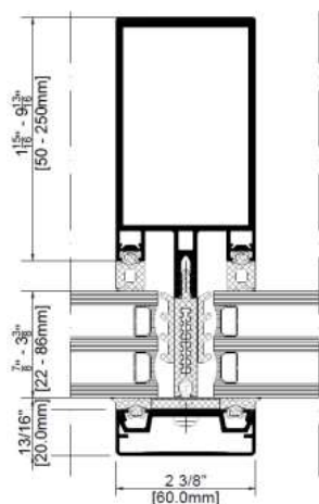
FWS 60.SI Mullion
