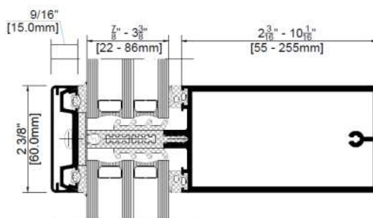
FWS 60.SI Transom
