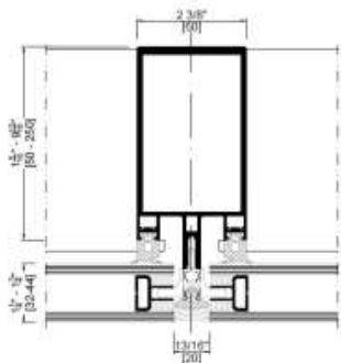
FWS 60 SG – Wet sealed
