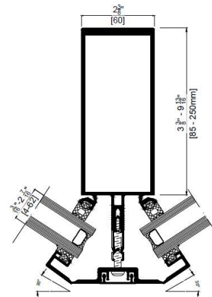
FWS 60 Corner Mullion
