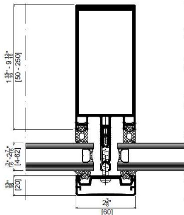
FWS 60 Mullion
