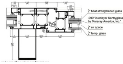
AWS 65 fixed and casement
