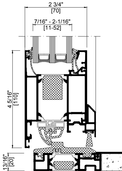
Sill section detail of Schüco AWS 70.HI Terrace Door
