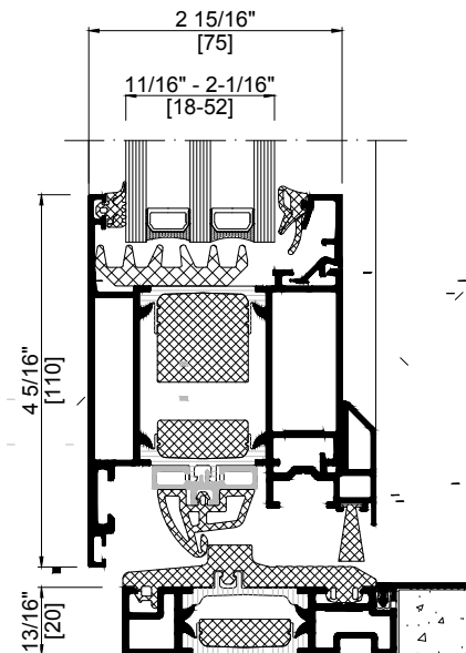
Sill section detail of Schüco AWS 75.SI+ Terrace Door
