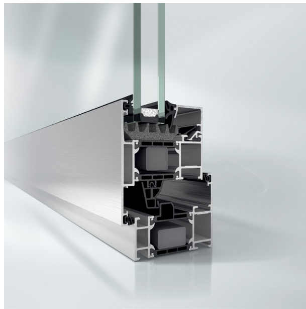
Schüco Window System AWS 70.HI, outward opening
