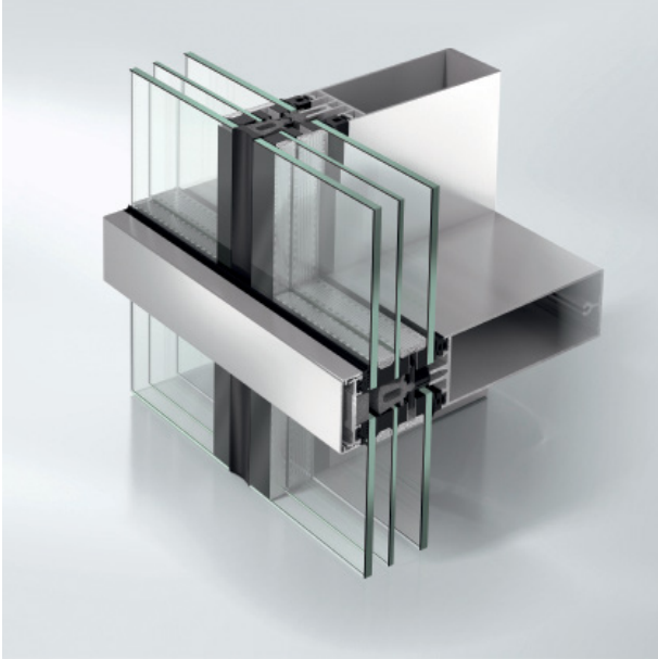
Schüco Facade System FWS 50 SG.SI with horizontal emphasis
